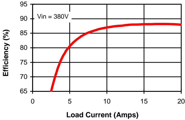
Efficiency
