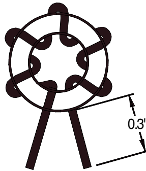
2uH, 15A Differential Choke
